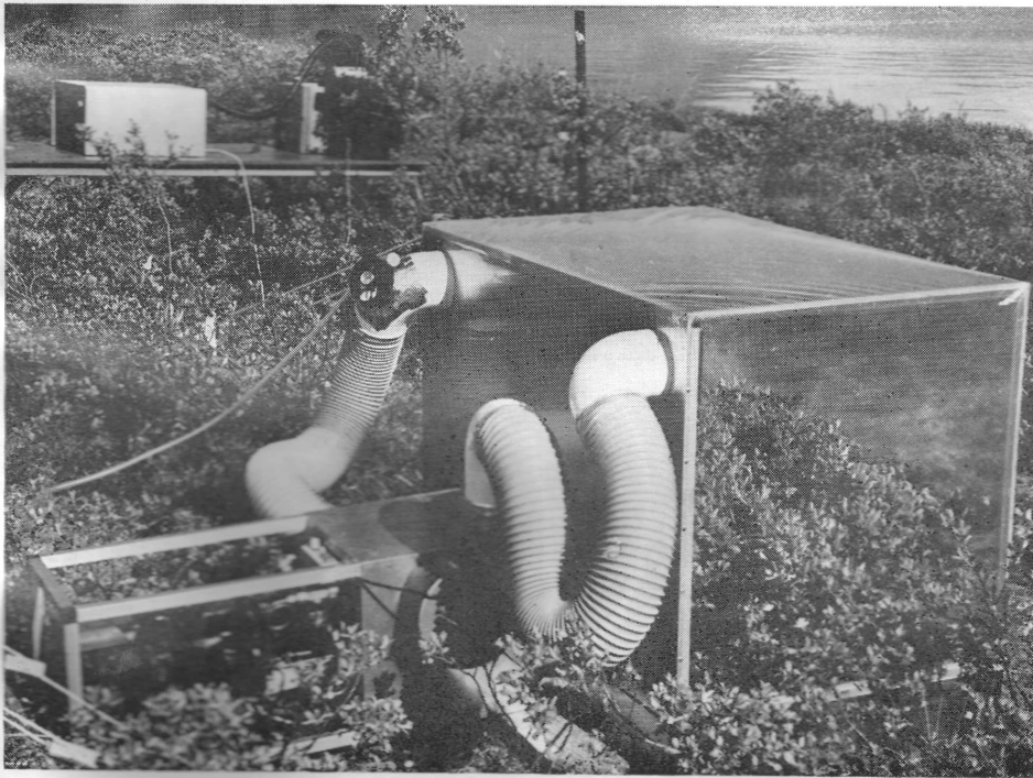
Fig. 6. Field station (top) including (a) infra-red gas analyser, logger and six point recorder, (b) meteorological mast, (c) net radiometer, (d) solarimeter, and (e-g) three controlled-environment plant-chambers. A 1 m 3 chamber set up in a Salix glauca stand in Kangerlussuaq (bottom).
